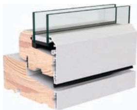
VELFAC Classic, 2-lags
